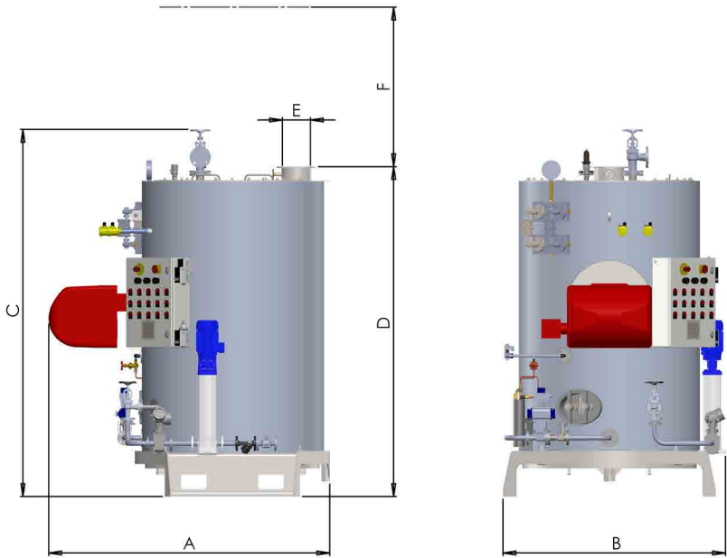
PEAKSMAN VERTICAL SERIES - BOILER DIMENSIONS
